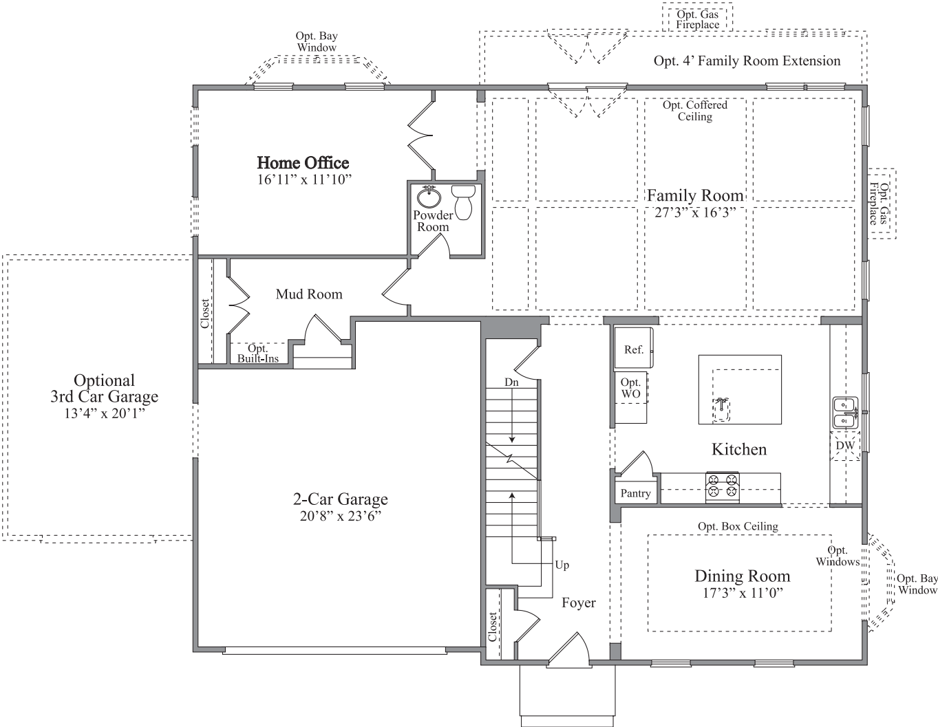
Main Level
